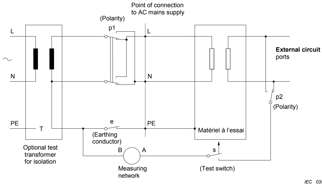
Figure 32 – Test circuit for touch current of single-phase equipment
