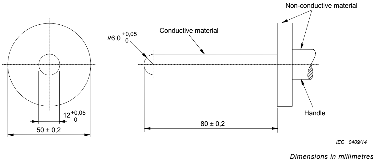
Figure V.3 – Blunt probe
